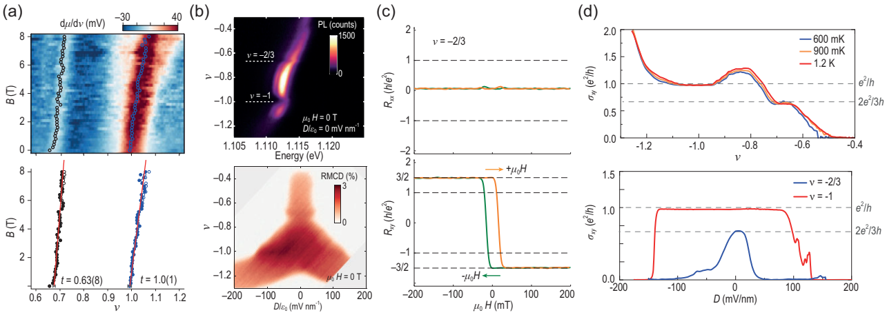
Figure 8. (a) Incompressibility measurement of twisted bilayer \text{MoTe}_2 . Integer (blue) and fractional (black) Chern insulators are respectively observed for hole fillings \nu = 1 and \nu = 2/3 . Adapted from [52]. (b) Trion photoluminescence exhibits blueshifts at \nu = -1 and \nu = -2/3 , respectively indicating integer and fractional Chern insulating states, which are also observable in the reflective magnetic circular dichroism measurement. Adapted from [51]. (c) Longitudinal and Hall resistances versus the magnetic field in twisted bilayer \text{MoTe}_2 . Plateaus are observed at R_{xy} = \pm 3h/2e^2 , corresponding to fractional filling \nu = -2/3 . Adapted from [53]. (d) Hall conductance versus filling/displacement in twisted bilayer \text{MoTe}_2 . Fractional Hall conductance \sigma_{xy} = 2e^2/3h is the smoking-gun evidence of fractional Chern insulators. Adapted from [54].
