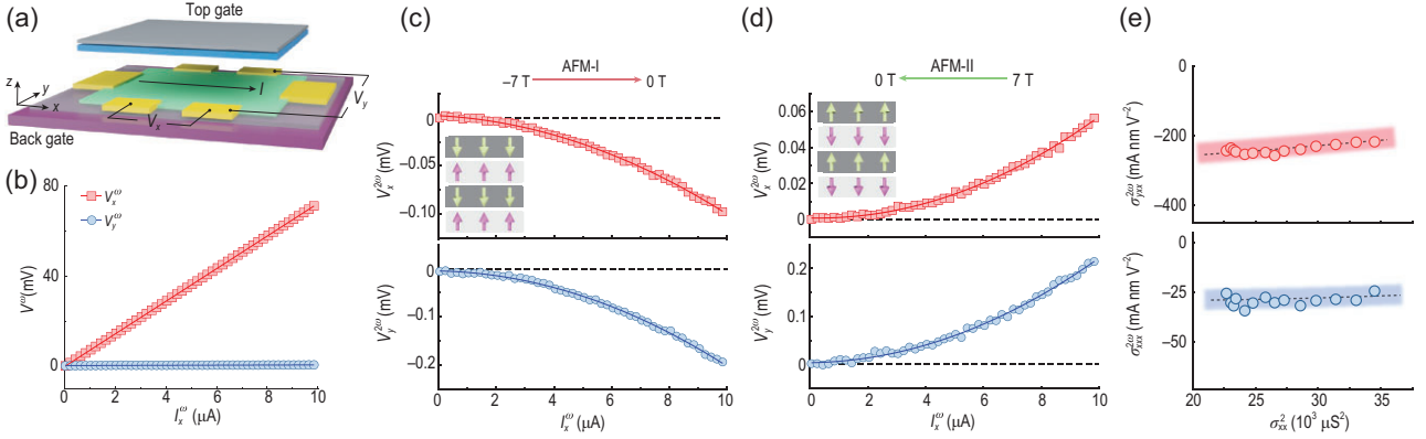
Figure 3. Electric nonlinear Hall effect and longitudinal conductivity. (a) Schematic plot of a six-end Hall bar device of four septuple-layer \text{MnBi}_2\text{Te}_4 (green) with a top gate (grey) and a back gate (purple). An ac driving current I^\omega is applied along the x direction, while linear/nonlinear voltages are measured along the x and y directions using the standard lock-in technique. (b) Linear longitudinal (red) and Hall (blue) voltages. (c),(d) Nonlinear longitudinal (red) and Hall (blue) voltages for the AFM-I and AFM-II phases of \text{MnBi}_2\text{Te}_4 . Insets illustrate the magnetization of each septuple layer in the AFM-I and AFM-II phases. (e) Scaling of the nonlinear Hall (red) and longitudinal (blue) conductivities with respect to the square of the linear longitudinal conductivity. The dashed lines are the linear fits according to Equation (20). All panels are adapted from [27].
