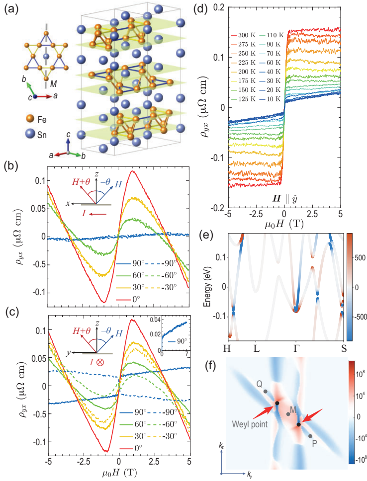
Figure 4. (a) Schematic atomic structure of \text{Fe}_3\text{Sn}_2 with gold (blue) balls representing iron (stannum) atoms. (b) Angle-resolved Hall resistivity for a magnetic field in the z - x plane. (c) Angle-resolved Hall resistivity for a magnetic field in the y - z plane. Inset: in-plane Hall resistivity occurs with a y -direction magnetic field. (d) Magnetic field dependence of Hall resistivity at different temperatures. (e) The yy component of the anomalous orbital polarizability projected onto the first-principles band structure. (f) Distribution of the anomalous orbital polarizability dipole on the Fermi surface, where a pair of Weyl points serve as the hot spots. All panels are adapted from [28].
